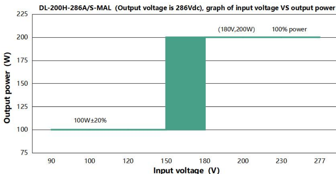
DL-200H-286A/S-MAL (For output 286Vdc, the rated output current & power under different input voltage)
