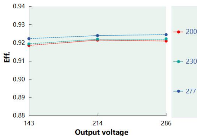
Eff. VS Output voltage(DL-200H-286A/S-MAL)
