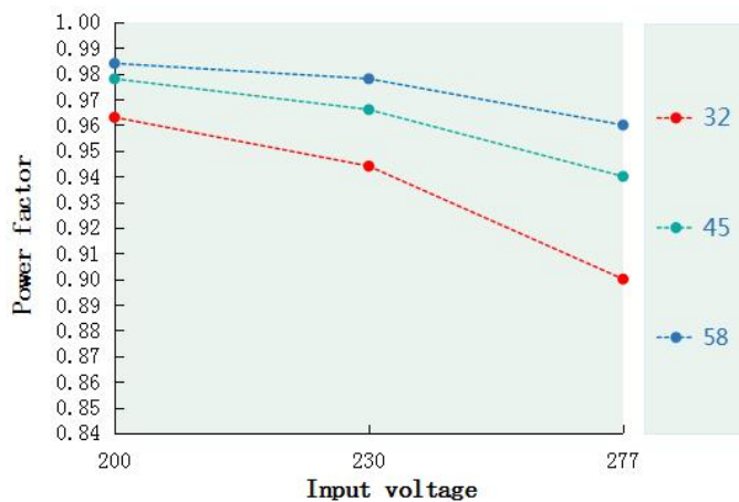
Power factor VS Input voltage(DL-200H-58A/S-MAL)
