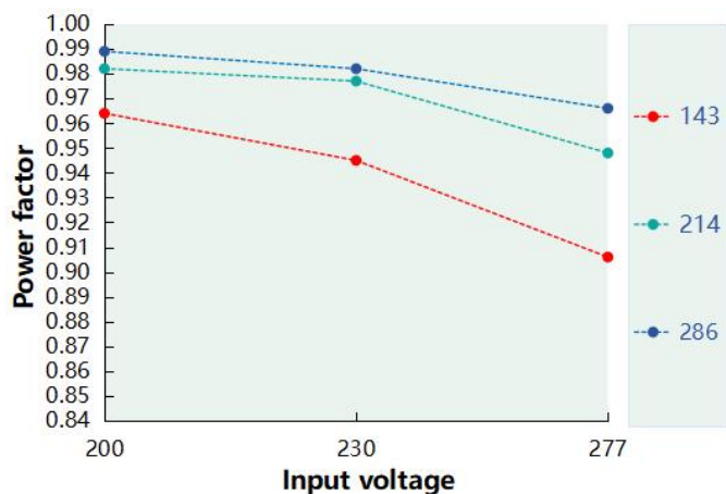
Power factor VS Input voltage(DL-200H-286A/S-MAL)
