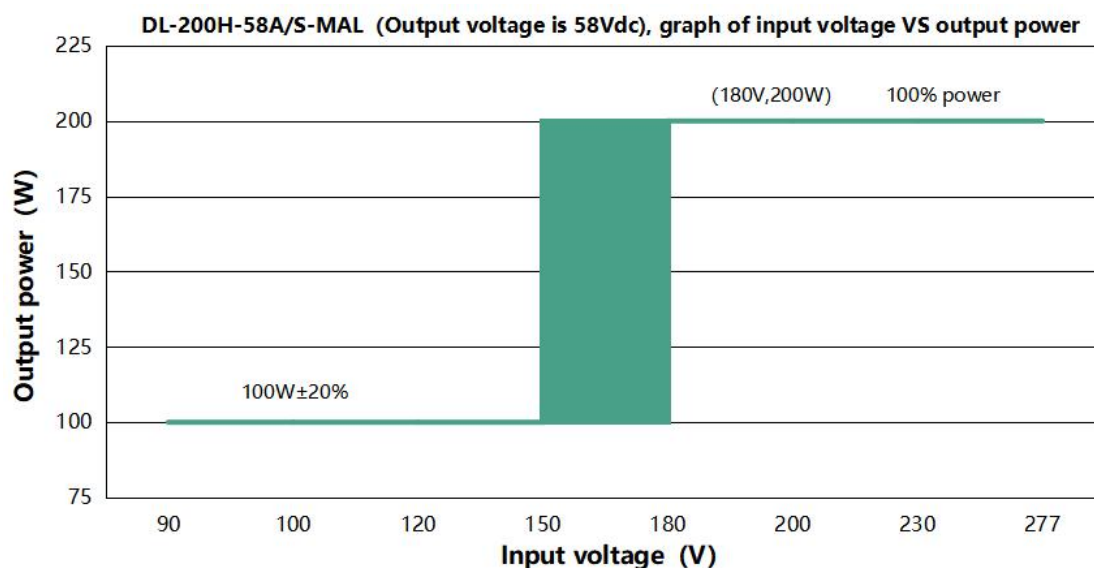
DL-200H-58A/S-MAL (For output 58Vdc, the rated output current & power under different input voltage)
