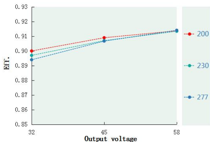
Eff. VS Output voltage(DL-200H-58A/S-MAL)
