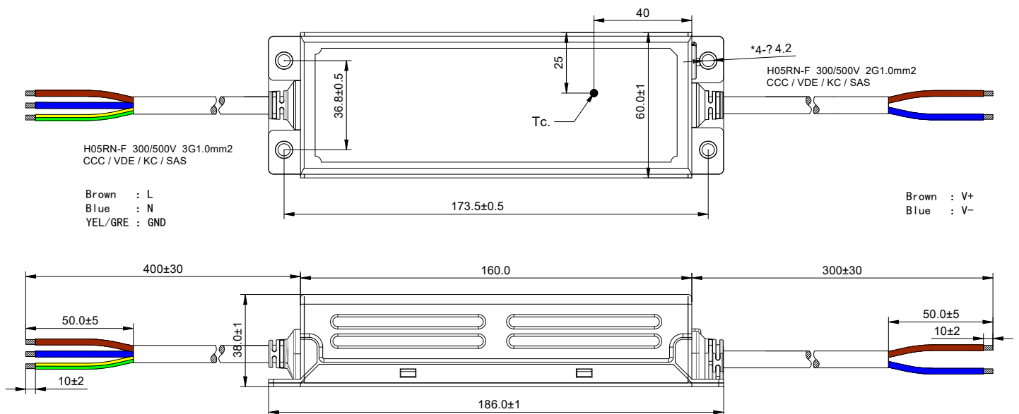
DL-200H-58A/286A-MAL
