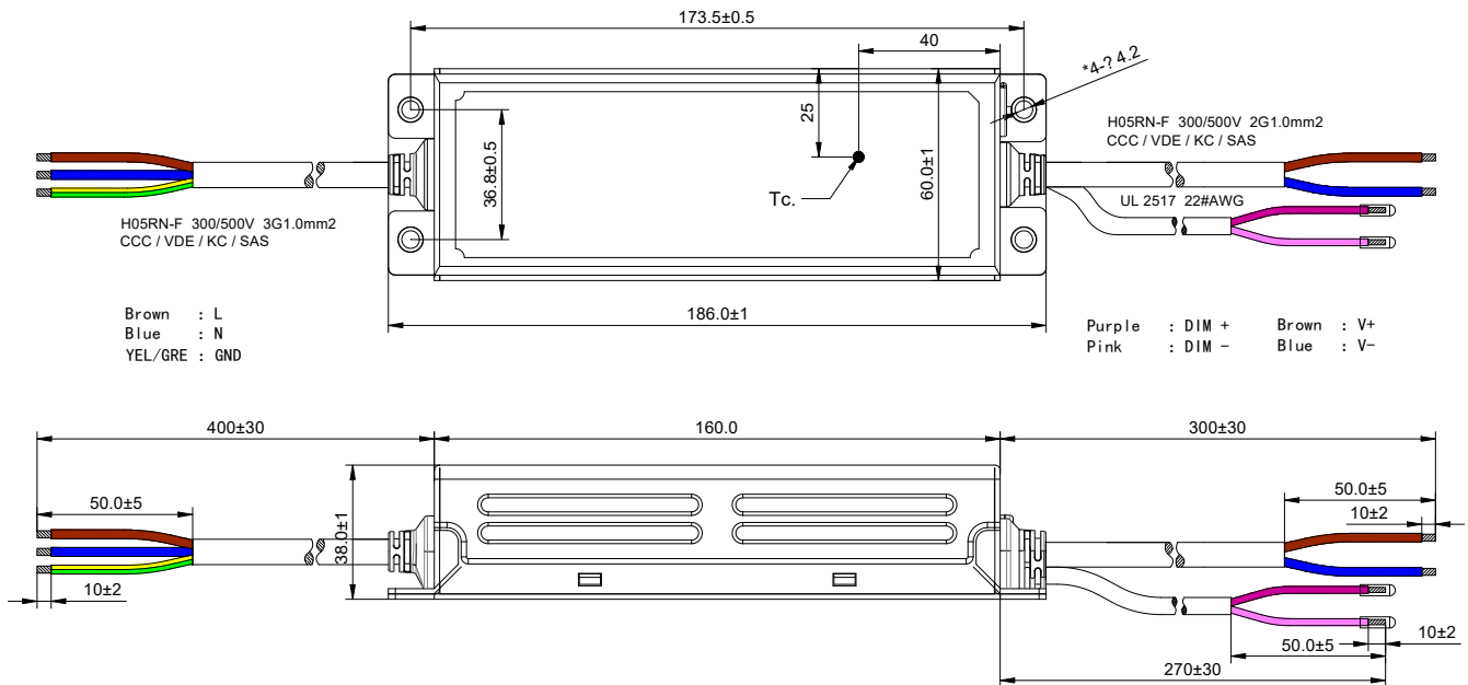
DL-200H-58S/286S-MAL
