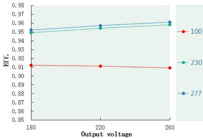
Eff. VS Output voltage (DL-240Z-260A/S/X -PXG)
