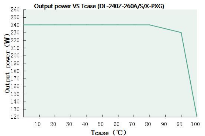
Output power VS Tcase (DL-240Z-260A/S/X -PXG)
