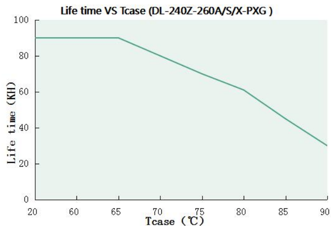
Lifetime VS Tcase (DL-240Z-260A/S/X -PXG)
