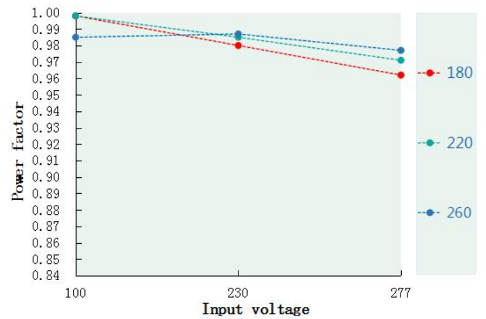
Power Factor VS Input Voltage (DL-240Z-260A/S/X -PXG)
