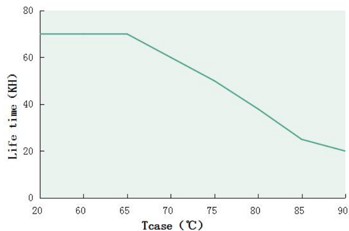
Tcase VS Lifetime(DL-50H-MAL)
