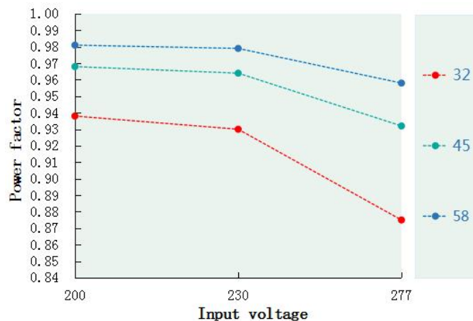
Power factor VS Input voltage(DL-50H-MAL)
