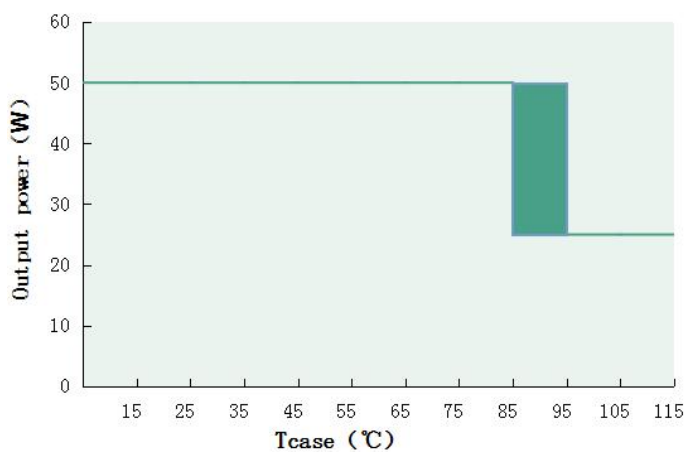
Output power VS Tcase (DL-50H-MAL)
